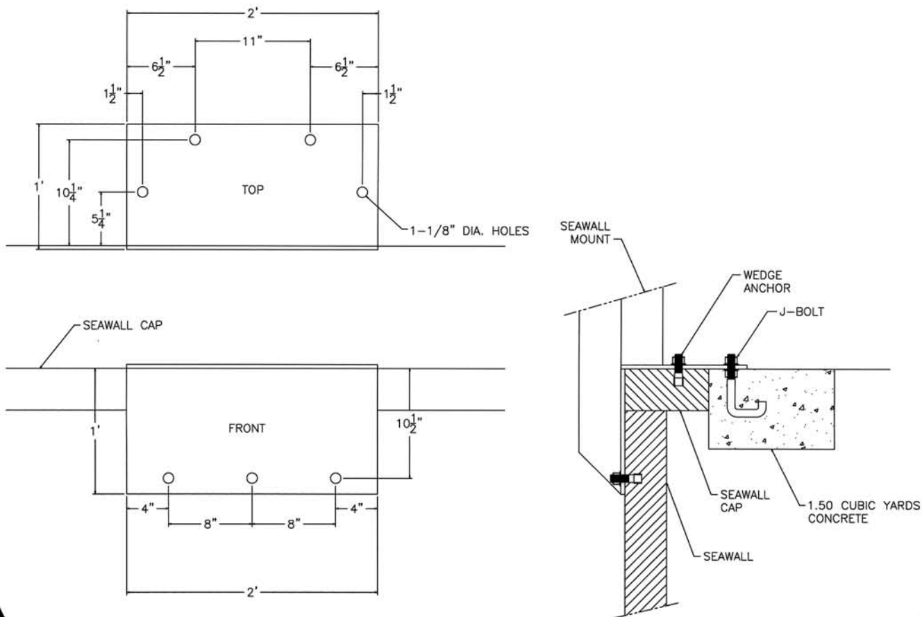
1,500 Lb. Spinner Seawall Mount Hole Layout
